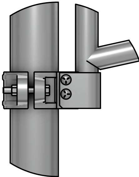
HINGE DETAIL B
